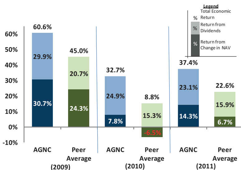
Figure 5: Economic Return
